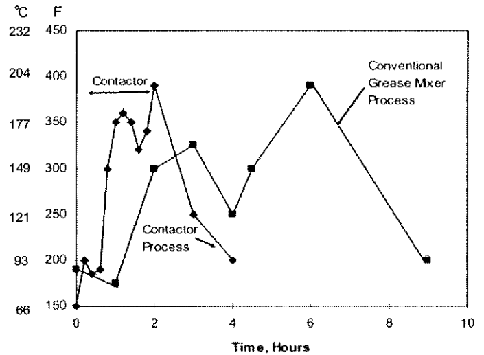
Time-Temperature Cycle for Lithium 12-Hydroxystearate Grease Manufactured in a Contactor Reactor
